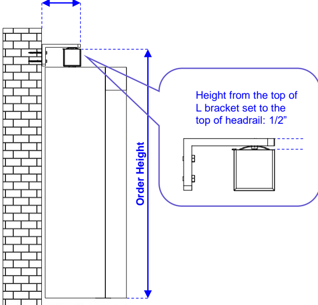
With Standard L Bracket Set
