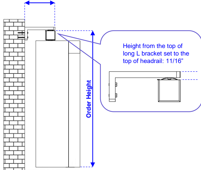
With Long L Bracket Set
