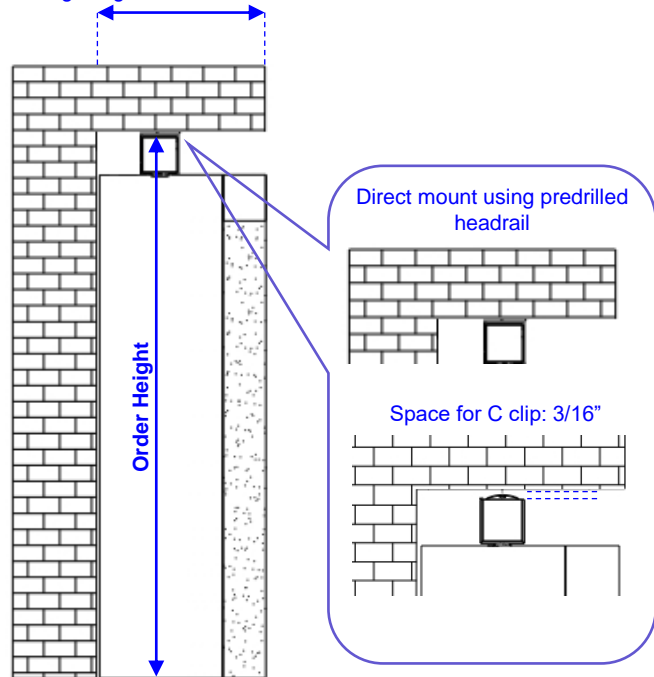
Fabric vane edge aligns with the wall
