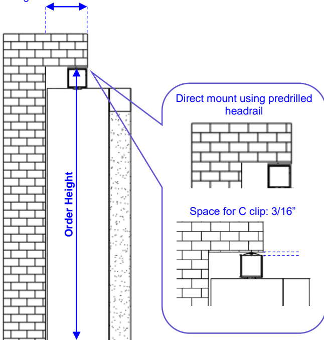
Headrail aligns with the wall
